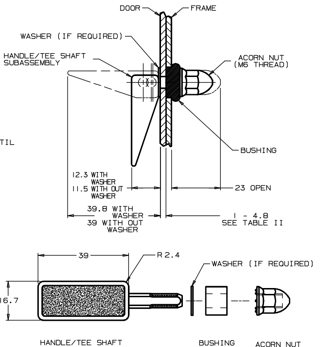
EXPLODED VIEW
